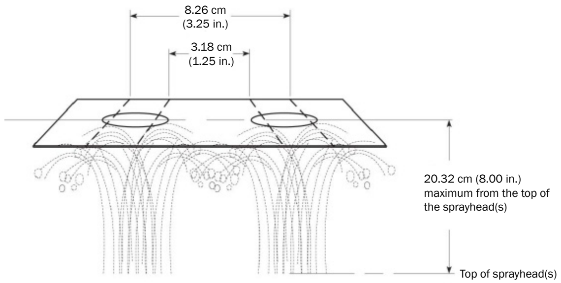
Illustration 4: Typical eyewash gauge
