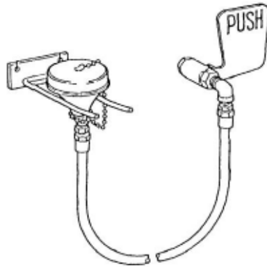
Illustration 9: Drench hose with eyewash attachment
